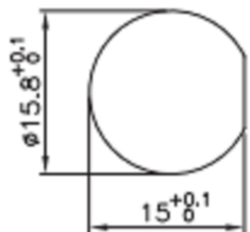
开孔尺寸 hole opening size
